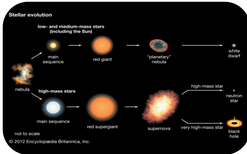
Figure 4: A star's evolution in time depends on its mass. (Credit: Encyclopædia Britannica)
