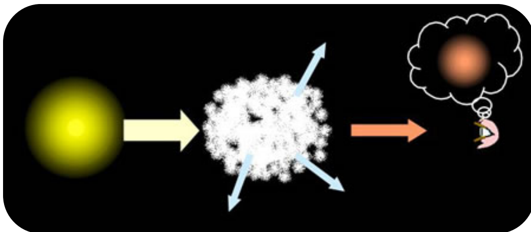
Figure 8: Dust grains along the line of sight scatter and absorb blue light and let red light get through. The object behind the dust will look redder and fainter than it really is. (Credit: COSMOS, the SAO Encyclopedia of Astronomy)
