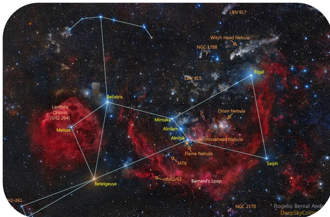
Figure 9: Giant molecular cloud in Orion. (Credit: Rogelio Bernal Andreo/DeepSkyColors.com)
