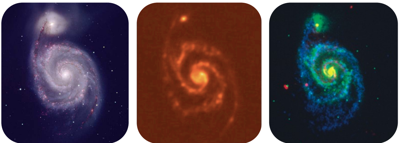
Figure 1: M51, the Whirlpool Galaxy, observed in visible light (Hubble Space Telescope, left), far-infrared (Herschel, centre) and radio (NRAO, right). (Credits: ESA/NASA/NRAO)
