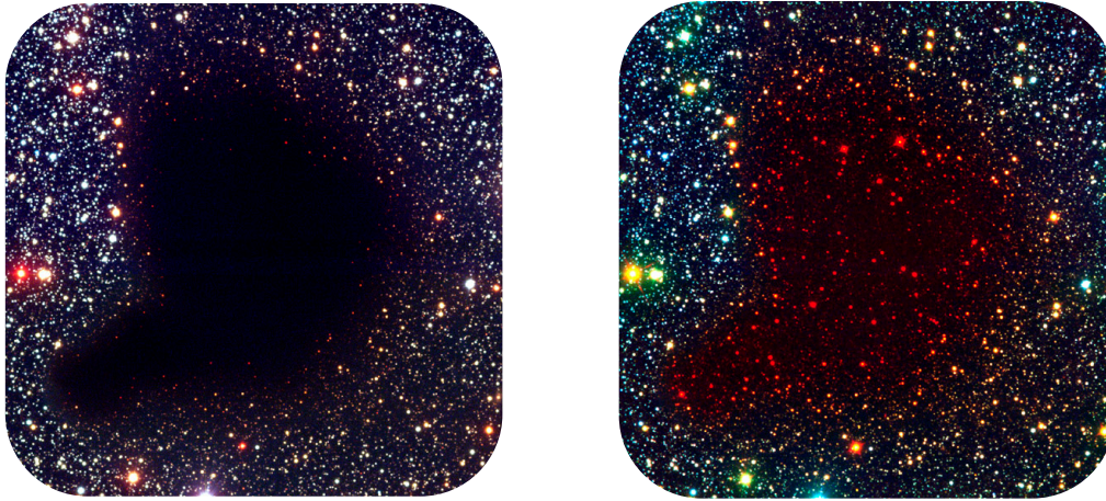
Figure 7: The left panel shows Barnard 68, a dark cloud, as it is observed in visible light. The right panel shows the image in the left combined with a near-infrared image of the same cloud, where the stars hidden in the dust are unveiled. (Credit: ESO)
