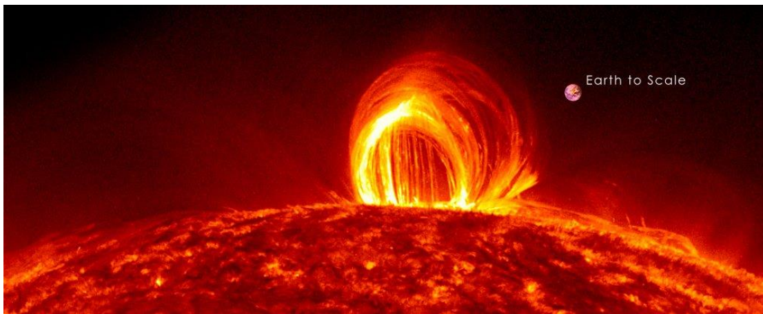
Figure 3: Solar "coronal rain" – some of the material released from a solar flare – falling back down to the Sun. Earth to Scale (Credit: NASA)
